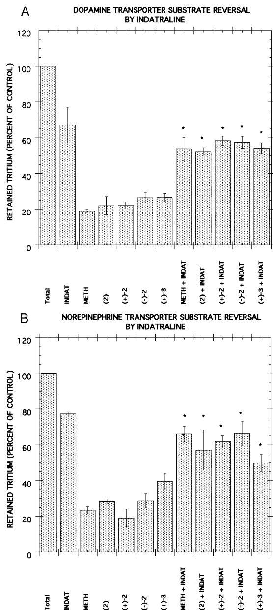
Fig. 4. Substrate activity of 2 , (+)- 2 , (–)- 2 , and (+)- 3 in the [ ^3 H]norepinephrine and [ ^3 H]dopamine release assays. Approximately ED_{80} concentrations of the test compound was tested in the absence and presence of 10 nM indatraline for activity in the [ ^3 H]dopamine (panel A) and [ ^3 H]norepinephrine (panel B) release assays. Each value is the mean \pm S.D. ( n=3 ). * p<0.05 when compared to the drugs alone (Student's t -test). Panel A: the drug concentrations were: indatraline (INDAT, 20 nM), (+)-methamphetamine (METH, 20 nM), 2 (500 nM), (+)- 2 (250 nM), (–)- 2 (1500 nM), (+)- 3 (5000 nM). Panel B: indatraline 200 nM, METH, 75 nM, 2 (250 nM), (+)- 2 (200 nM), (–)- 2 (250 nM), (+)- 3 (2000 nM).
