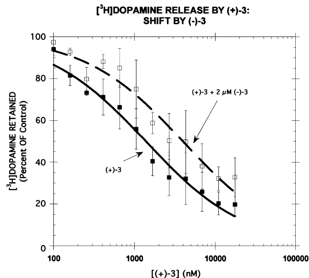
Fig. 5. Dopamine transporter substrate activity of (+)-pseudophenmetrazine ((+)- 3 ). (+)- 3 dose–response curves in the [ ^3 H]dopamine release assay were generated in the absence ( EC_{50} = 1384 nM) and presence of 2 \mu M (–)- 3 ( EC_{50} = 3976 nM). Each value is the mean \pm S.D. ( n=3 ).
